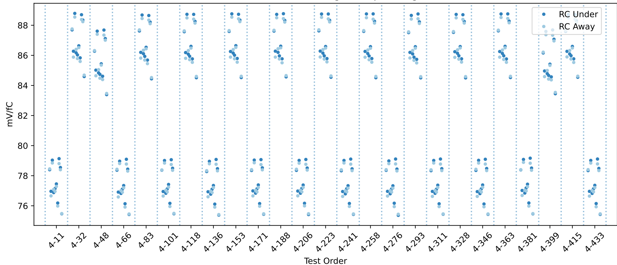
20USBHX2003346 RC gain chip averages
