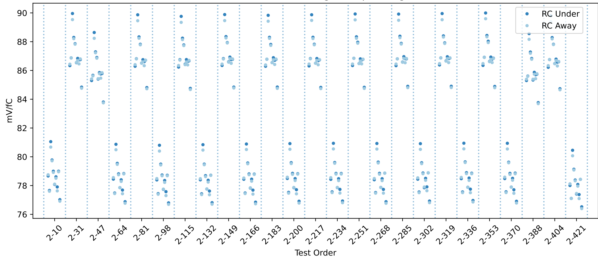
20USBHX2003462 RC gain chip averages
