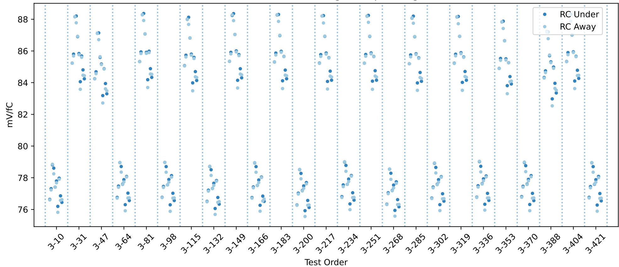
20USBHX2003464 RC gain chip averages
