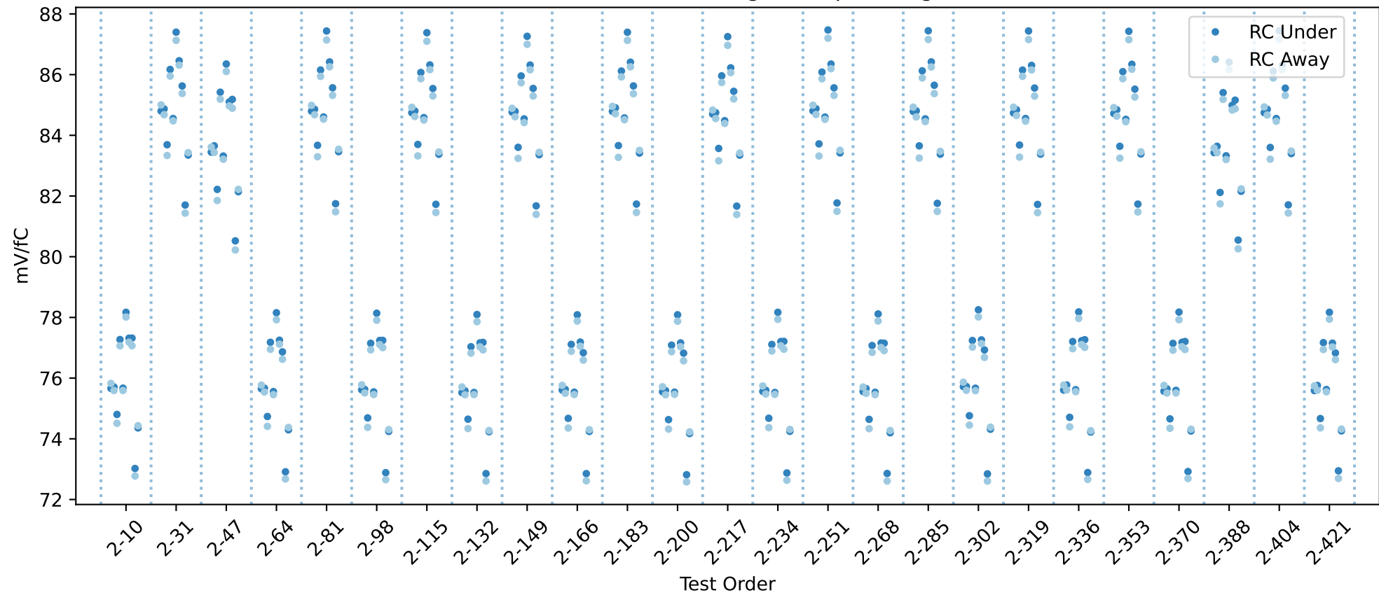
20USBHX2003364 RC gain chip averages
