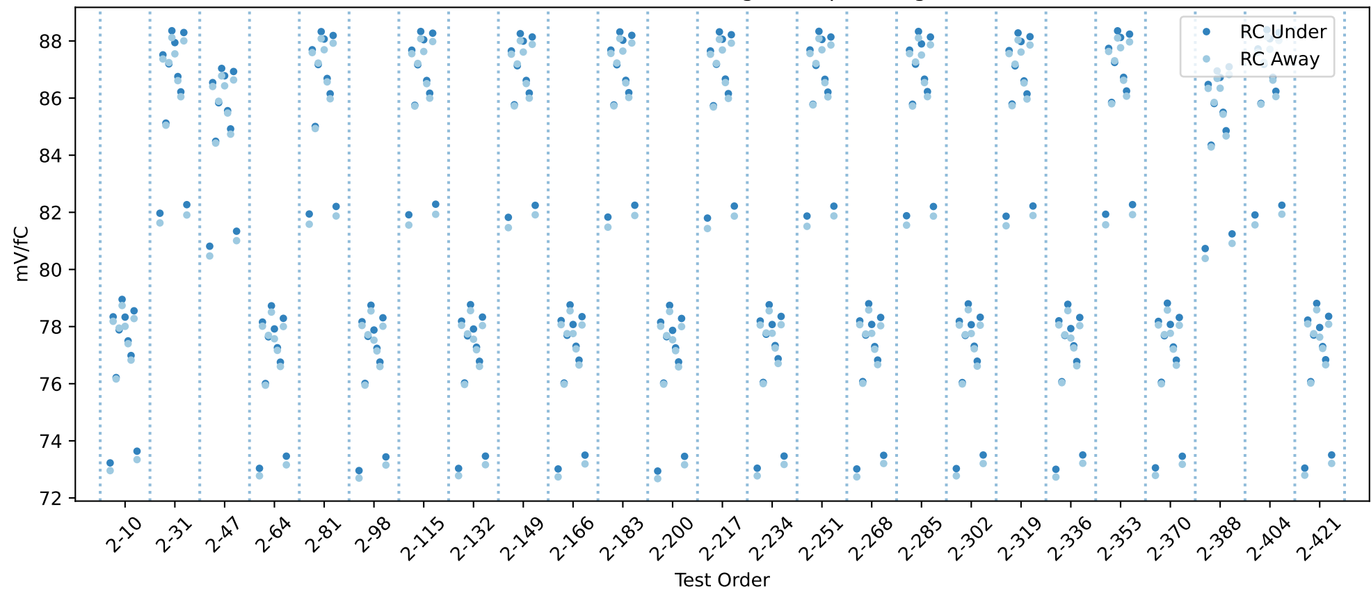
20USBHX2003366 RC gain chip averages
