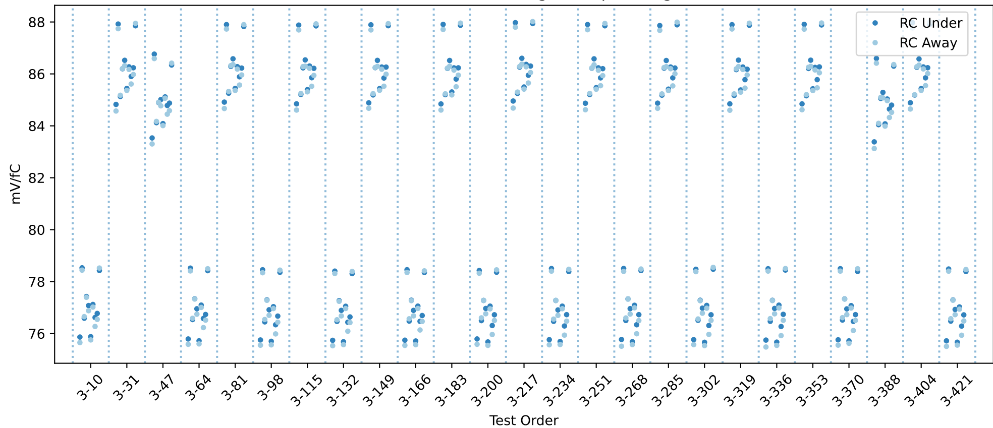
20USBHX2003588 RC gain chip averages
