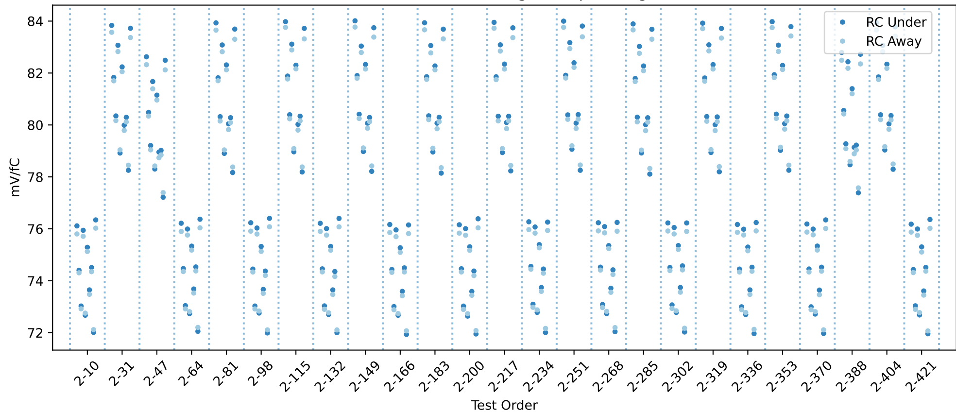
20USBHX2003577 RC gain chip averages
