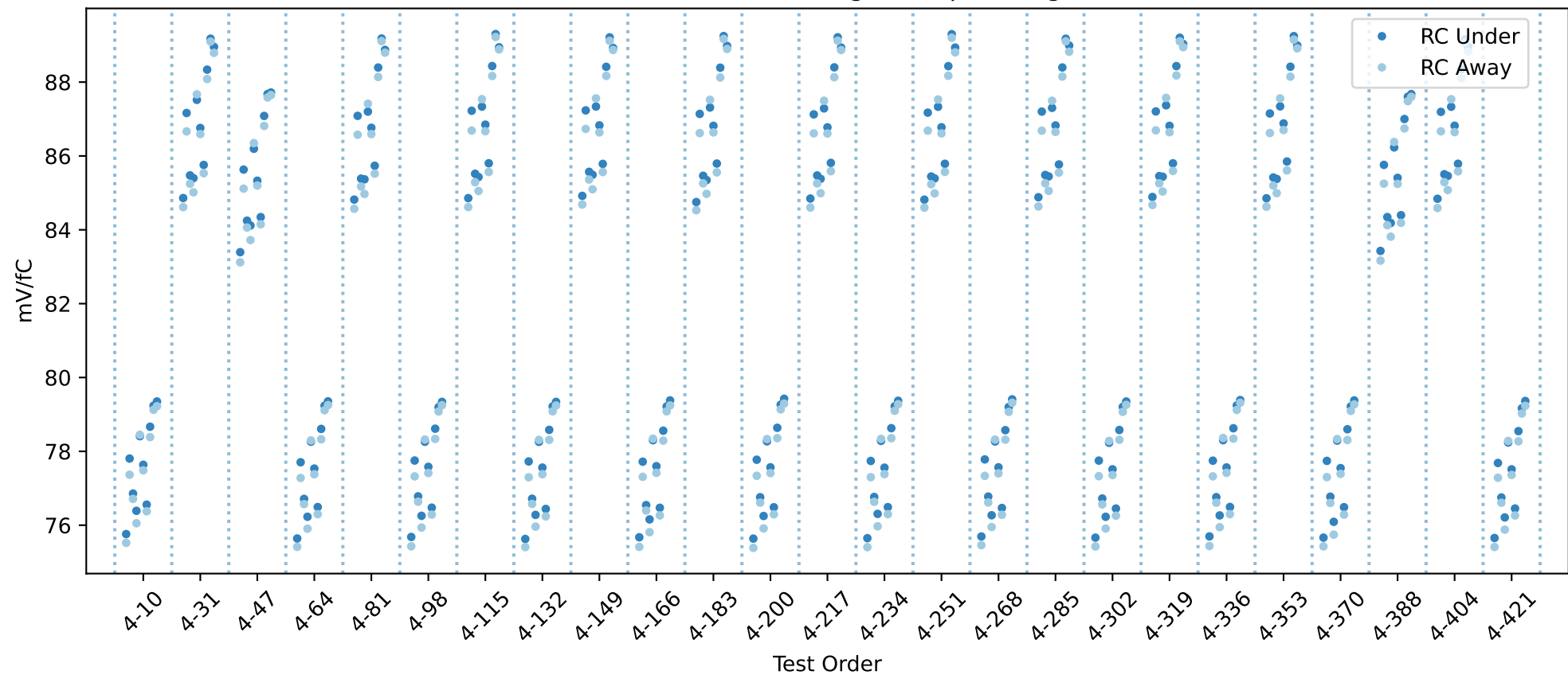
20USBHX2003595 RC gain chip averages
