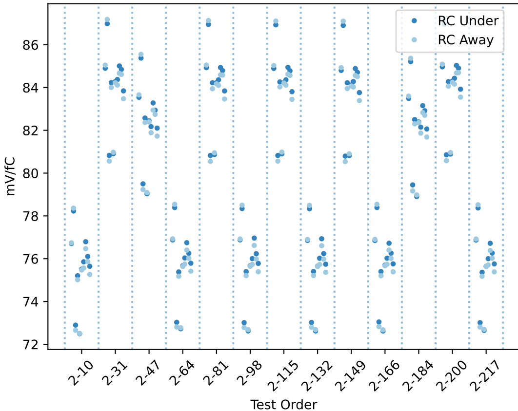
20USBHX2001986 RC gain chip averages
