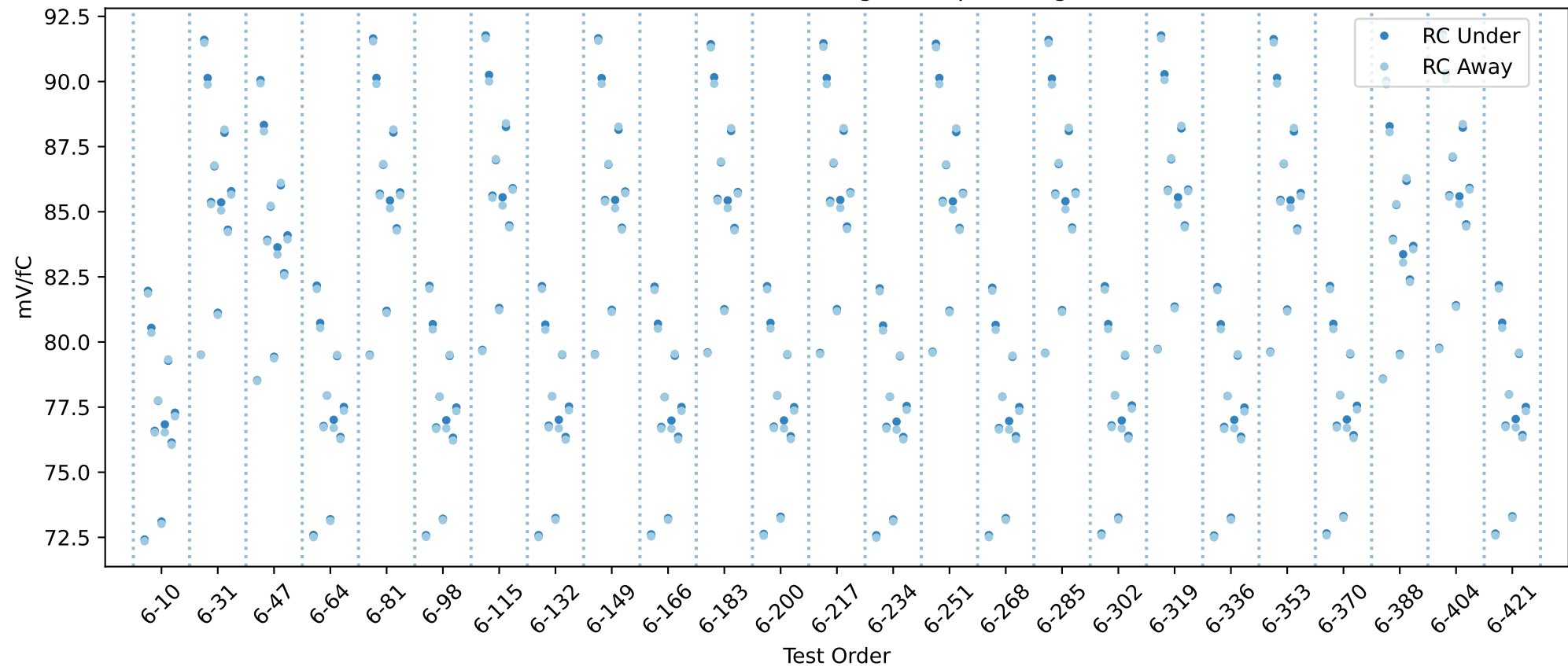
20USBHX2001939 RC gain chip averages
