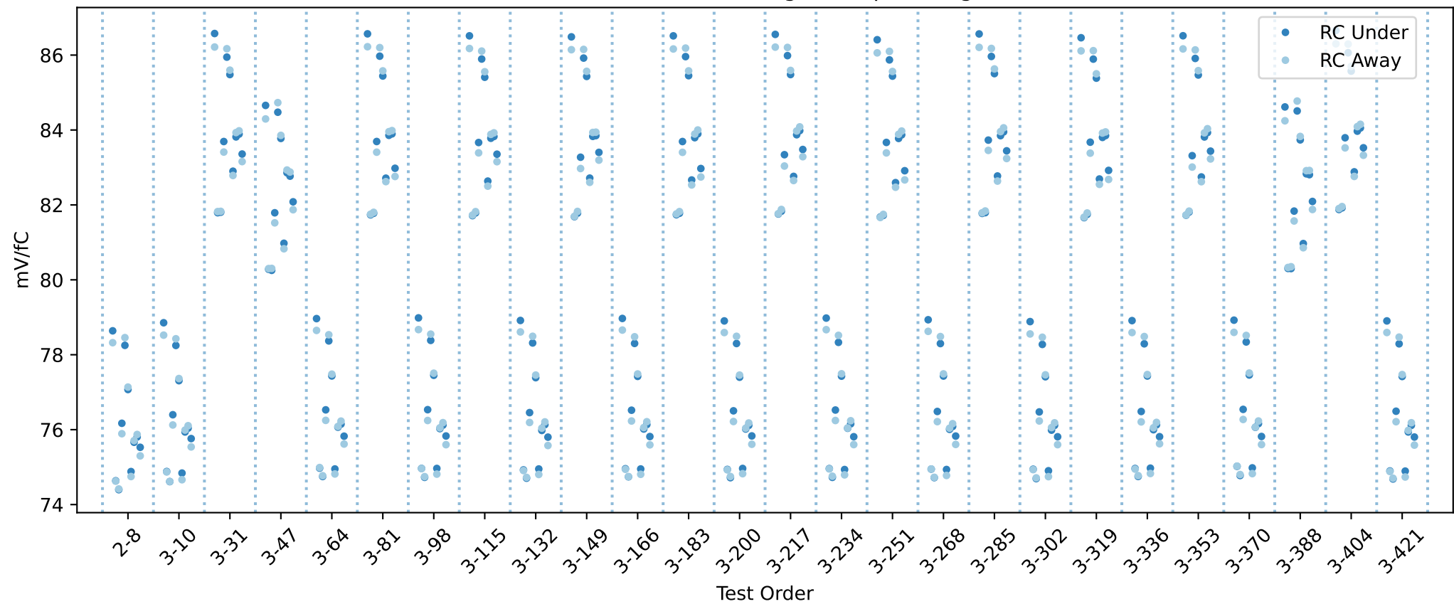
20USBHY0000561 RC gain chip averages
